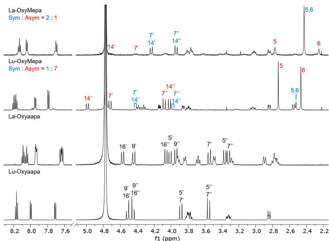
Figure 2. ^1\text{H} NMR spectra of OxyMepa and Oxyaapa complexes formed with \text{La}^{3+} and \text{Lu}^{3+} (600 MHz, \text{D}_2\text{O} , pD = 7, 25 °C). Diagnostic peaks are labeled, and the numbering scheme is shown in Chart 2. The high-intensity peak near 4.8 ppm arises from residual H 2 O in the NMR solvent.
