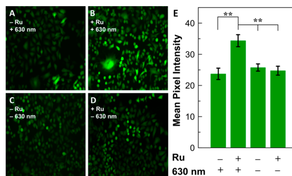
Figure 4. Images of \text{H}_2\text{S} release from [\mathbf{1}]\text{Cl} . A549 cells were incubated with 5\ \mu\text{M} SF7-AM for 30 min, washed and then (A) exposed to red light for 30 min; (B) treated with 60\ \mu\text{M} [\mathbf{1}]\text{Cl} and exposed to red light for 30 min; (C) incubated for 30 min in the dark; (D) treated with 60\ \mu\text{M} [\mathbf{1}]\text{Cl} for 30 min in the dark. (E) Mean pixel intensity of fluorescence images for A549 cells in the experiments described in panels A–D. Error bars are SE of n = 5 or 6 wells from two biological replicates. Statistical significance was determined using a two-tailed student's t test. **p < 0.005 .
