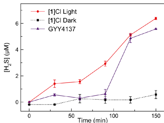
Figure 3. \text{H}_2\text{S} release from [\mathbf{1}]\text{Cl} ( 200\ \mu\text{M} ) with red light irradiation (red circles), [\mathbf{1}]\text{Cl} ( 200\ \mu\text{M} ) in the dark (black squares), and GYY4137 ( 200\ \mu\text{M} ) (purple triangles) measured by DNS-az fluorescence. Errors bars are the standard error (SE) of three independent trials.
